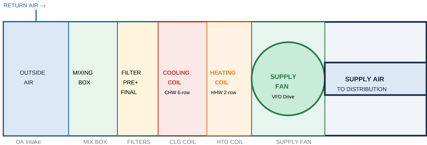
Figure 1 — Typical AHU Section Assembly (Not to Scale)
